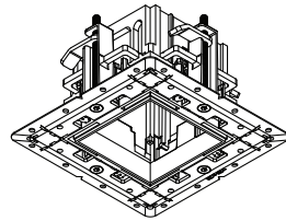
Qbini trimless frame 1x (141800XX)
